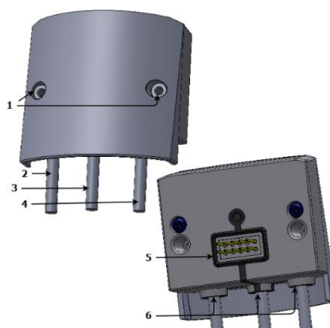
Fig. 3. Structure of the APT-ELF2-MBUS-2 module
