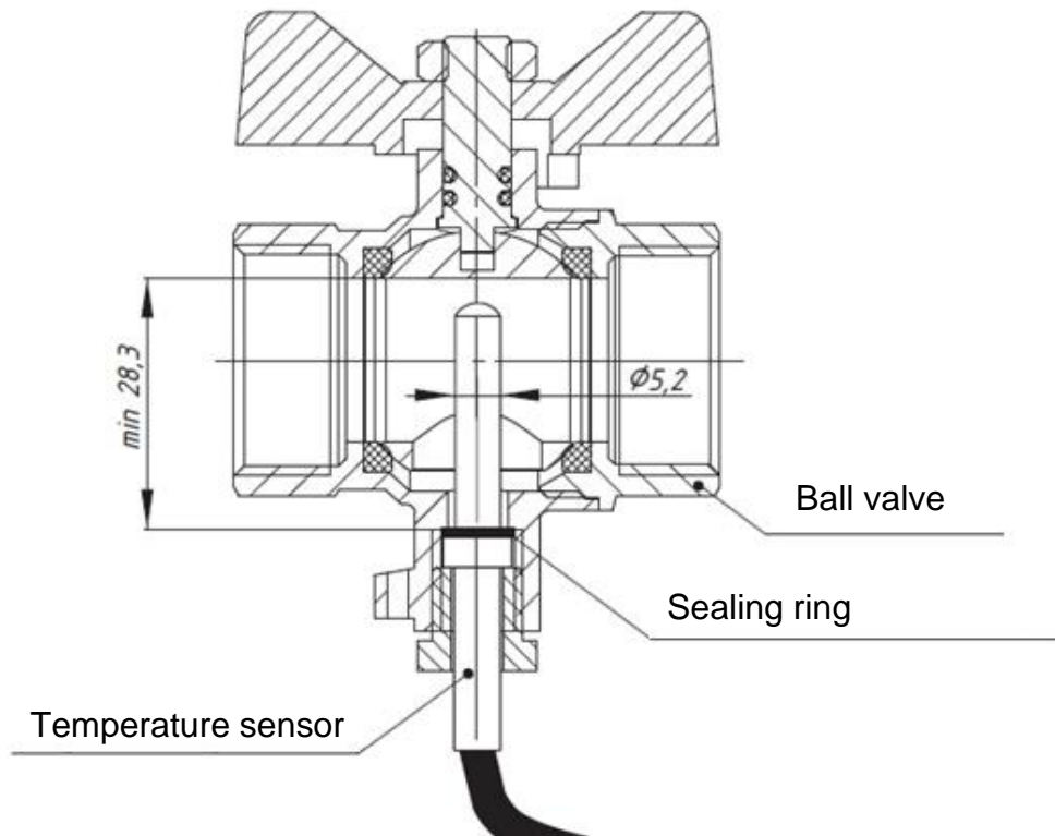
Fig.9. Temperature sensor installation in a ball valve
