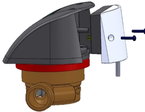
Fig.7. Module installation
