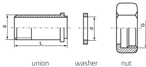
Connection fittings
